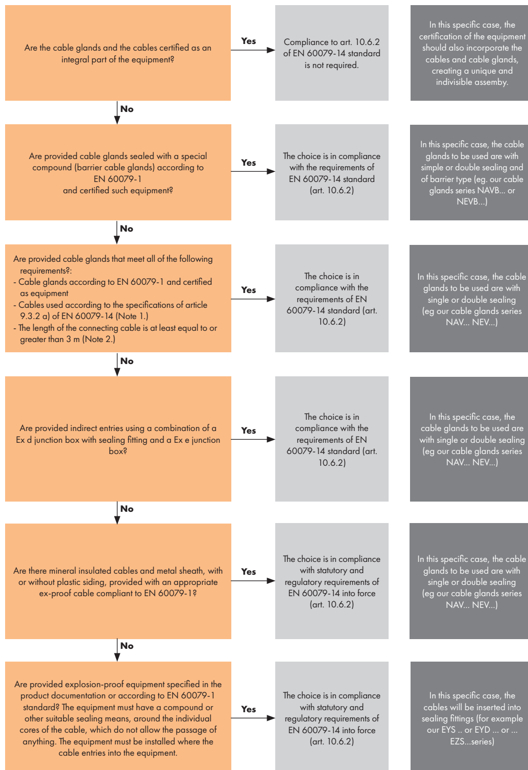
FIG.8 Flow chart for the correct selection of the cable entry in Ex d junction boxes
